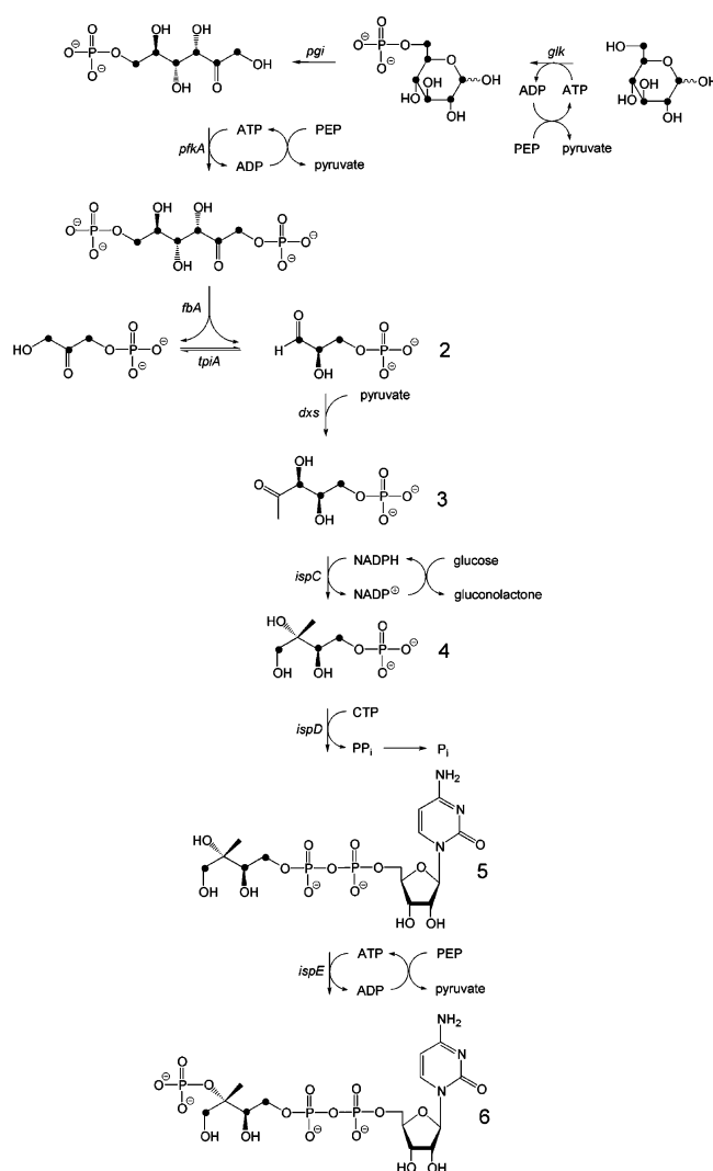
FIGURE 2. Synthesis of [1,3,4- 13 C 3 ]4-diphosphocytidyl-2C-methyl-D-erythritol 2-phosphate ( 6 ) from [U- 13 C 6 ]glucose. 13 C-atoms are indicated by full circles.
