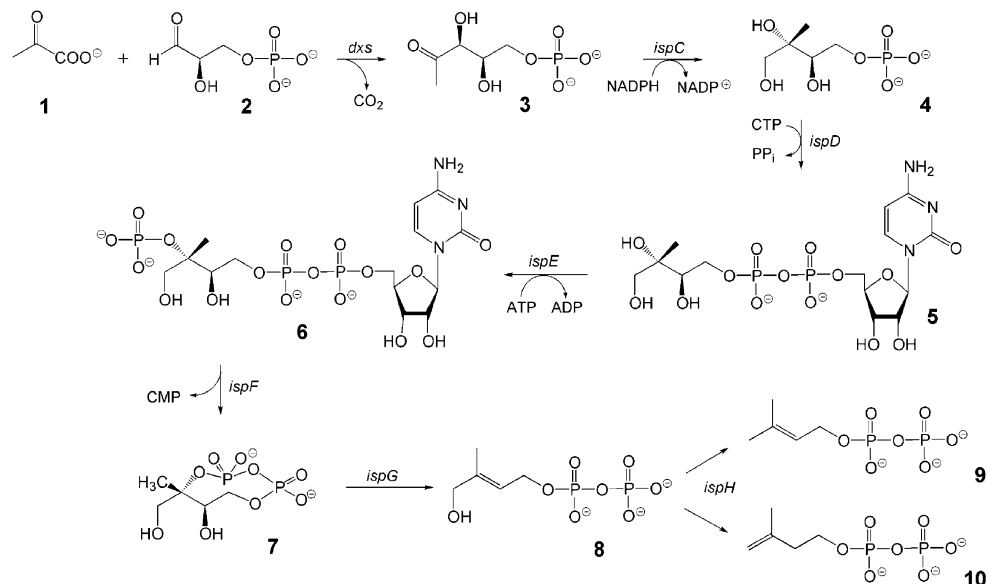
FIGURE 1. Nonmevalonate isoprenoid pathway.
