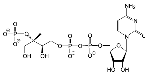
4-Diphosphocytidyl-2C-methyl-D-erythritol 2-phosphate
