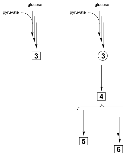
FIGURE 3. Flux diagram for synthesis and isolation procedures of nonmevalonate isoprenoid pathway intermediates. Symbols: ○, removal of protein by ultrafiltration; □, product purification.
